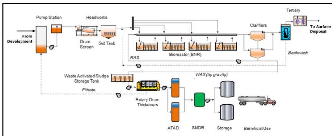
Figure 3 – Midhurst WWTP Process Flow Diagram
