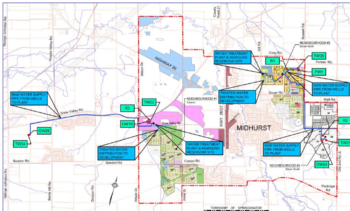
Figure 2 – Water Solution Recommended by Class EA
