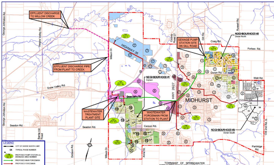
Figure 2 – Wastewater Solution Recommended by Class EA
